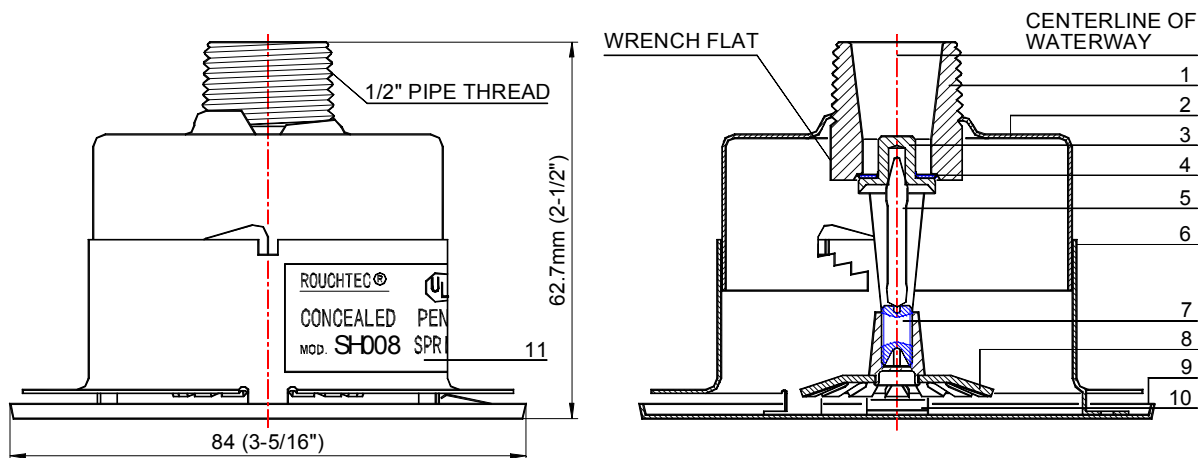
FIGURE A : MODEL SH007/SH008 CONCEALED PENDENT SPRINKLER
