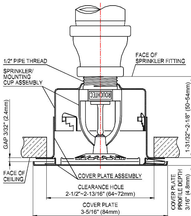
FIGURE E : MODEL SH007/SH008 CONCEALED PENDENT SPRINKLER TYPICAL INSTALLATION
