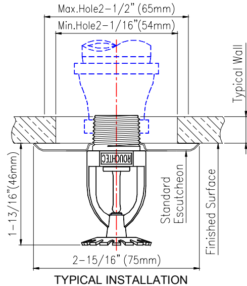
FIGURE C : MODEL SH005/SH006 PENDENT SPRINKLER INSTALLED WITH A STANDARD ESCUTCHEON
